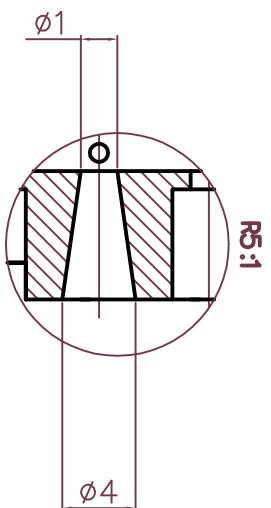
detail A
